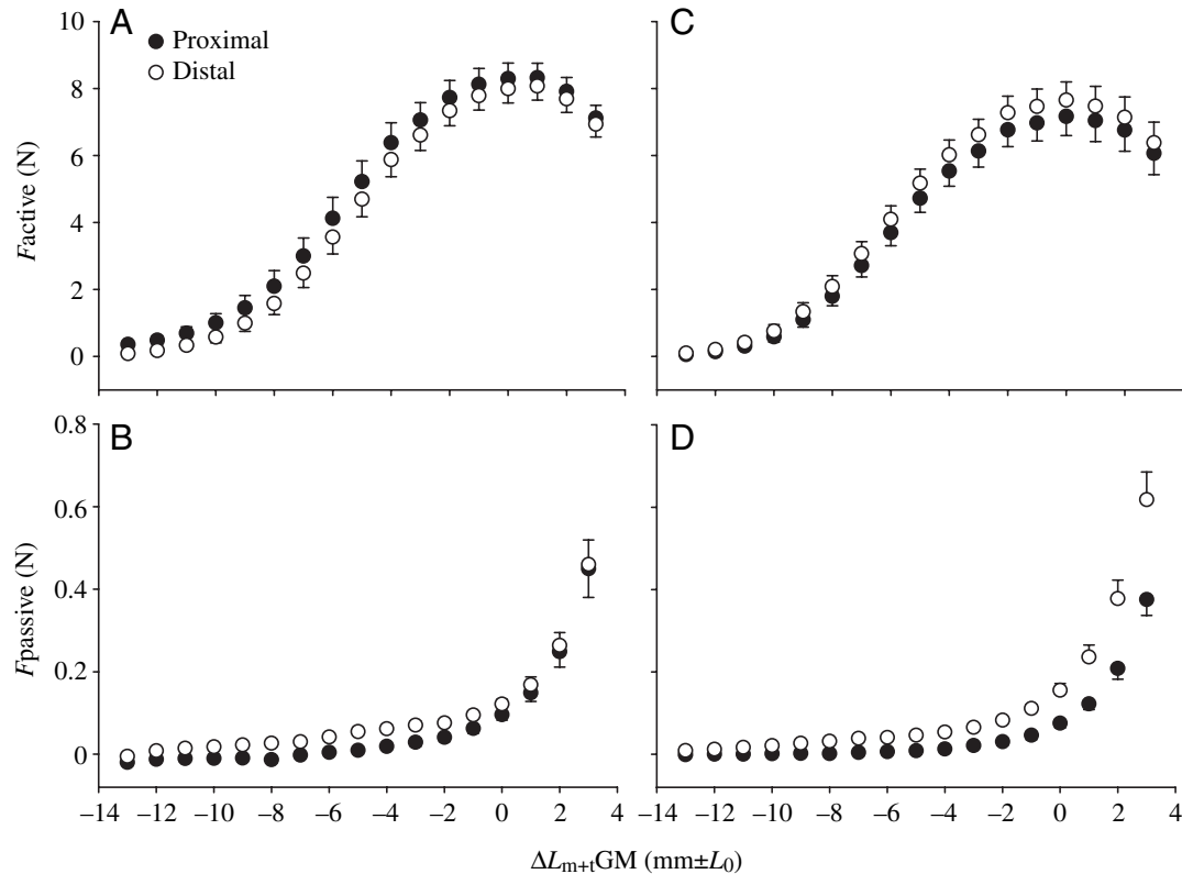
Fig. 8. Effects of muscle relative position of fully dissected in situ rat medial gastrocnemius (GM) muscle on force. Muscle relative position was manipulated by moving the origin 3 mm proximally or distally from the reference position (i.e. the position corresponding to a knee angle of 120°). (A) Active force–length characteristics after moving the origin in the proximal direction. (B) Passive force–length characteristics after moving the origin in the proximal direction. (C) Active force–length characteristics after moving the origin in the distal direction. (D) Passive force–length characteristics after moving the origin in the distal direction. Proximal and distal forces (mean \pm S.E.M.) are represented by closed and open symbols, respectively. Muscle–tendon complex length ( L_{m+t} ) is expressed as deviation from optimum length ( L_0 ).
