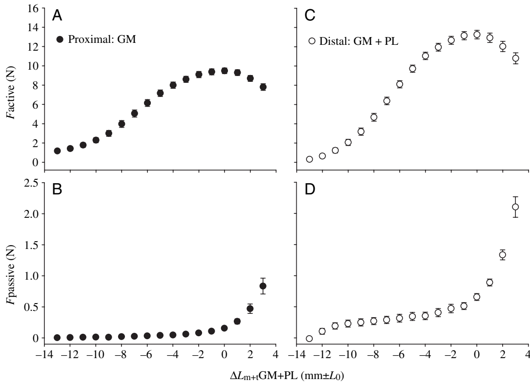
Fig. 3. Forces exerted at the proximal and distal transducers by rat medial gastrocnemius (GM) and plantaris (PL) muscles connected to extramuscular connective tissue at the level of the tendons and the muscle bellies (initial condition), within a dissected compartment. (A,B) Proximal active and passive force exerted at the GM tendon. (C,D) Distal active and passive force exerted at the calcaneal bone. Proximal force (closed symbols) represents force exerted predominantly by the GM muscle. Distal force (open symbols) represents predominantly the summed force exerted by the GM and PL muscles. Note that, at short lengths, the summed distal active force was lower than the proximal active force. Muscle–tendon complex length ( L_{m+t} ) is expressed as deviation from optimum length ( L_0 ). Force is shown as mean \pm S.E.M.
