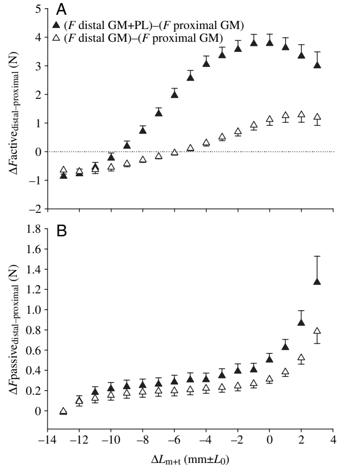
Fig. 5. Effect of distal plantaris-tenotomy on proximo–distal force differences. (A) Proximo–distal active force differences. (B) Proximo–distal passive force differences. Closed symbols represent the data before tenotomy (i.e. both medial gastrocnemius (GM) and plantaris (PL) distal tendons connected to calcaneal bone). Open symbols represent post-tenotomy data. Note that a substantial fraction of PL force was still transmitted to the distal force transducer. Muscle tendon complex length ( L_{m+t} ) is expressed as deviation from optimum length ( L_0 ). Force is shown as mean \pm S.E.M.
