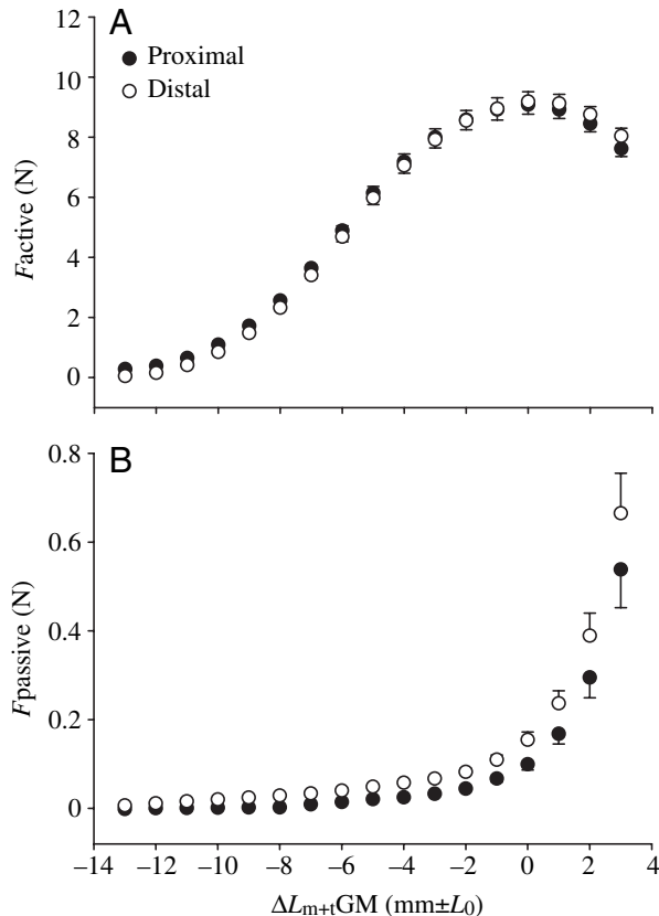
Fig. 6. Force-length characteristics of partially dissected rat medial gastrocnemius (GM) muscle connected only at the level of the muscle belly by extramuscular connective tissue (i.e. remnants of the general fascia and epimysium). (A) Active forces exerted at the proximal tendon (closed symbols) and at the distal tendon (calcaneal bone) (open symbols). (B) Passive forces exerted at the proximal tendon (closed symbols) and at the distal tendon (calcaneal bone) (open symbols). Muscle-tendon complex length ( L_{m+t} ) is expressed as deviation from optimum GM muscle-tendon complex length ( L_0 ). Force is shown as mean \pm S.E.M.
