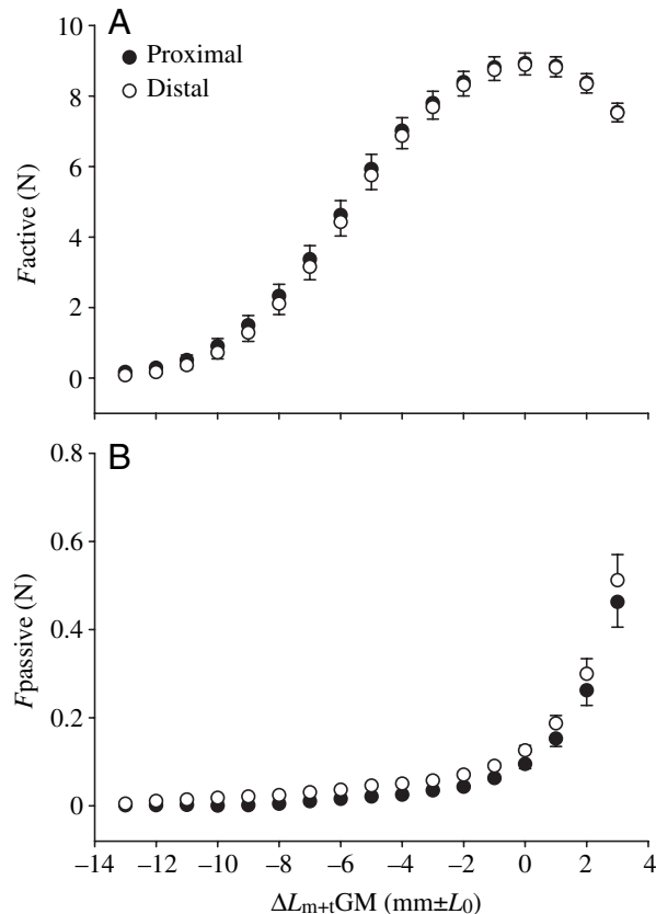
Fig. 7. Force-length characteristics of fully dissected rat medial gastrocnemius (GM) muscle with only the neuro-vascular tract as extramuscular connective tissue. GM had been dissected free from extramuscular tissues except for its innervation, blood supply and associated connective tissues. (A) Active forces exerted at the proximal tendon (closed symbols) and at the distal tendon (calcaneal bone) (open symbols). (B) Passive forces exerted at the proximal tendon (closed symbols) and at the distal tendon (calcaneal bone) (open symbols). Muscle-tendon complex length ( L_{m+t} ) is expressed as deviation from optimum GM muscle-tendon complex length ( L_0 ). Force is shown as mean \pm S.E.M.
