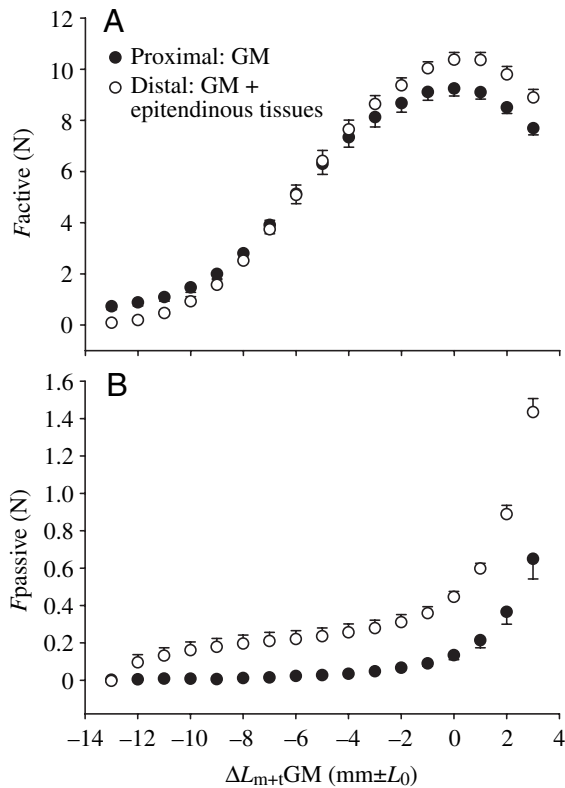
Fig. 4. Forces exerted at the proximal and distal transducers by rat GM and PL muscles connected to extramuscular connective tissue, within a dissected compartment after distal PL-tenotomy. Note that after distal PL-tenotomy, epitendinous tissues connected to the calcaneal bone were left intact. (A) A comparison of proximal active force exerted at the GM tendon (closed symbols) and distal active force exerted at the calcaneal bone (open symbols). (B) A comparison of proximal passive force exerted at the GM tendon (closed symbols) and distal active force exerted at the calcaneal bone (open symbols). Note that, despite PL-tenotomy, distal active force was higher at long muscle lengths and lower at short muscle lengths than proximal active force. Distal passive force was higher than proximal passive force. Muscle-tendon complex length ( L_{m+t} ) is expressed as deviation from optimum length ( L_0 ). Force is shown as mean \pm S.E.M.
