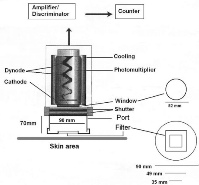
Fig. 1. Schematic representation of the photomultiplier device including the port extension, square frame for use of coloured glass filters.
